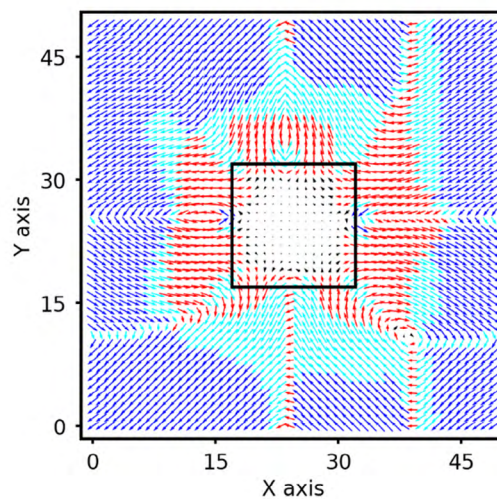
Figure 1. Local polarization profile around 6 nm \text{SrTiO}_3 inclusion (solid square in the middle) embedded in a \text{BaTiO}_3 matrix. Colors encode tetragonal (red), orthorhombic (cyan) and rhombohedral (blue) phases.
